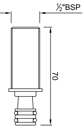
SPOUT NIPPLE
