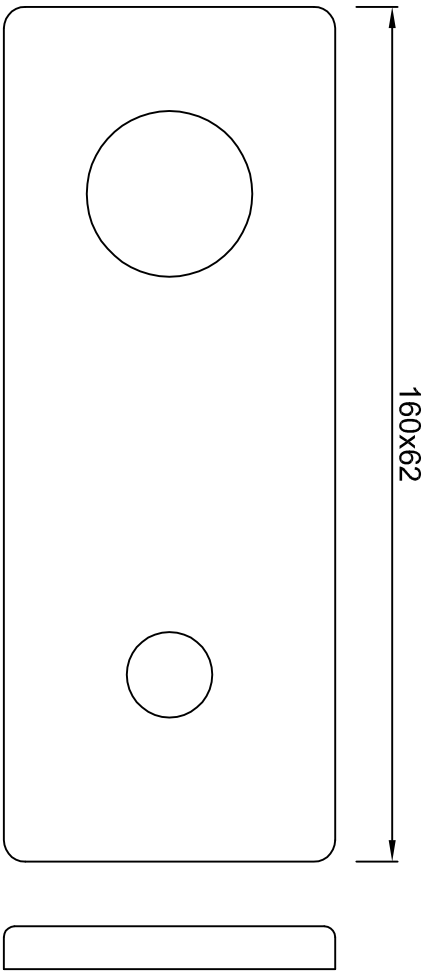
WALL FLANGE
