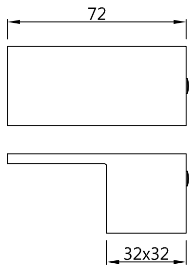
HANDLES
