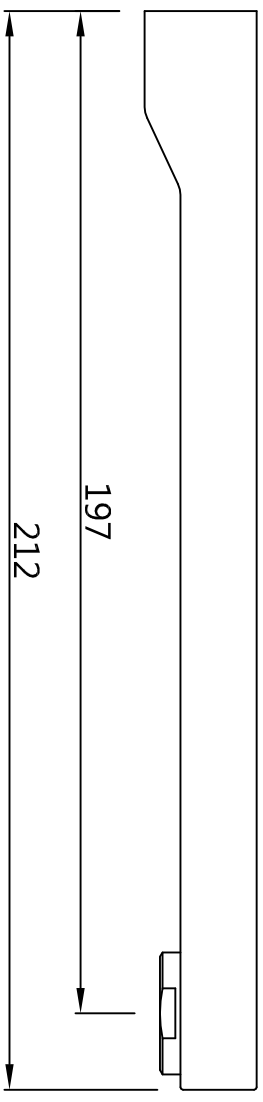
SPOUT
