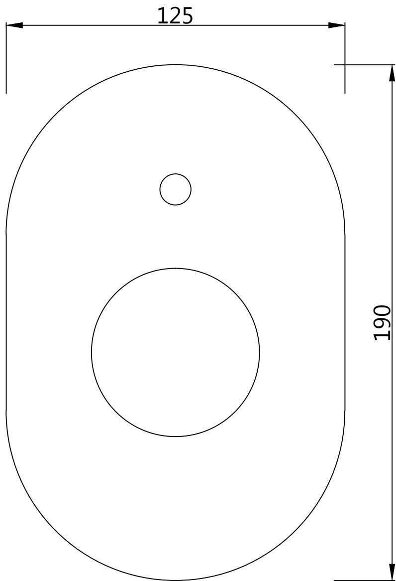
WALL FLANGE
