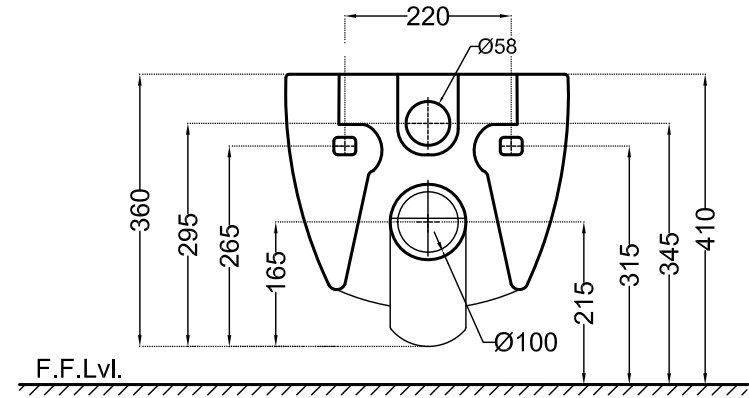
BACK VIEW
