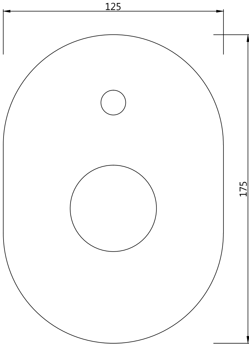
WALL FLANGE
