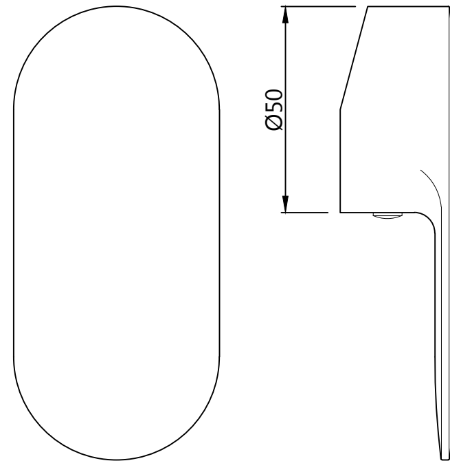
HANDLE
