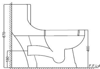
SIDE SECTION
